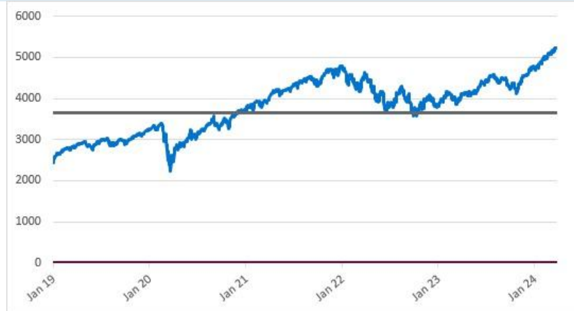
SPX Daily Index Closing Values January 2, 2019 to March 25, 2024
