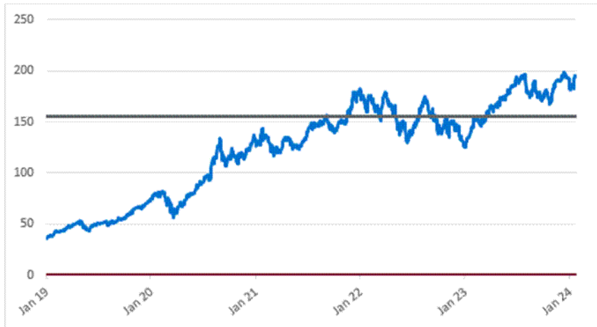
Common Stock of Apple Inc. – Daily Closing Prices January 2, 2018 to January 24, 2024
