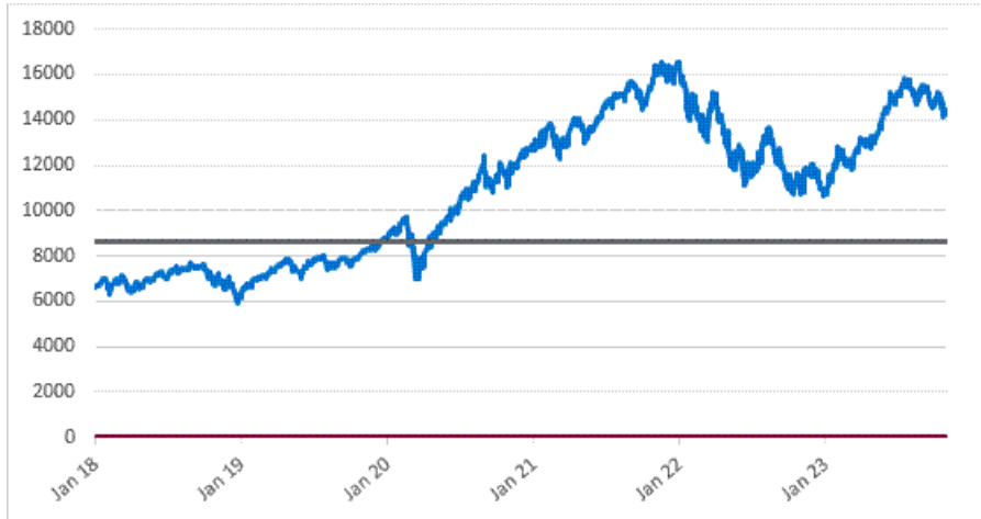
NDX Daily Closing Values January 2, 2018 to October 31, 2023
