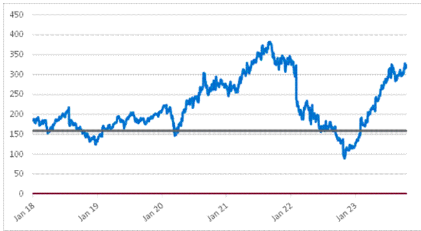
Class A Common Stock of Meta Platforms, Inc. – Daily Closing Prices January 2, 2018 to October 27, 2023
