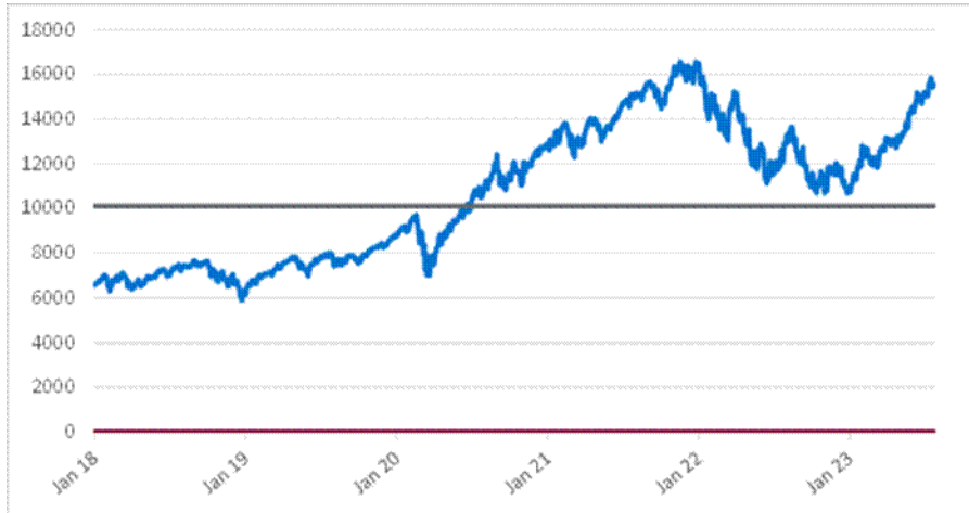
NDX Daily Closing Values January 2, 2018 to July 25, 2023
