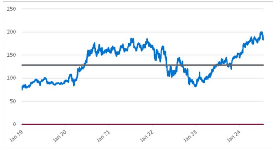
Common Stock of Amazon.com, Inc. – Daily Closing Prices January 2, 2019 to July 19, 2024
